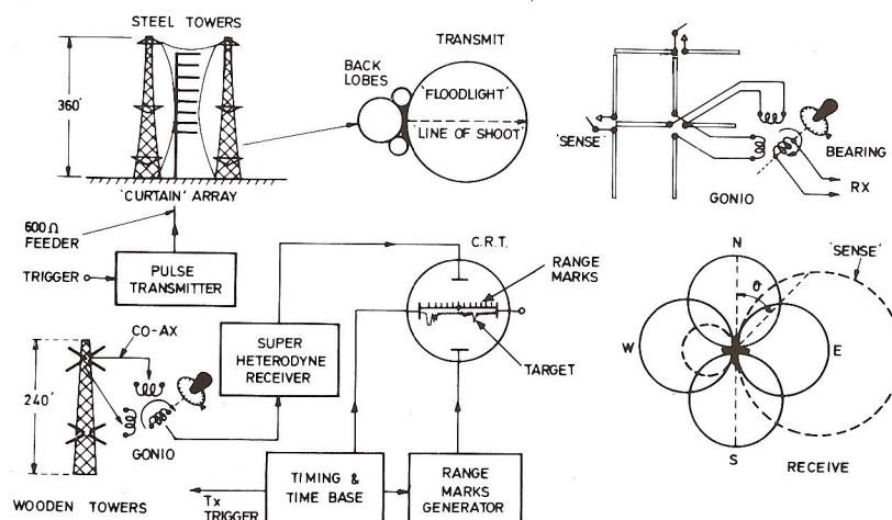
Fig. 1. Principles of CH (Chain Home) R.D.F. system
