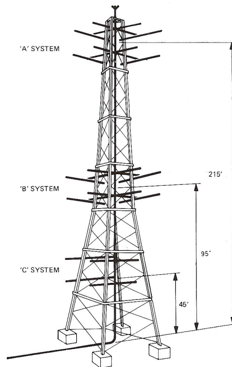
Fig. 8. Dipole arrays on a receiver tower
