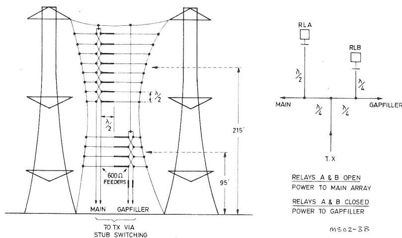
Fig. 3. (a) CH transmitter array (b) stub switching
