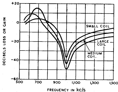
Fig. 3 (Above) Practical curves showing performance of wavetraps with various \frac{L_1}{C_1} ratios. All traps were adjusted so as to reject 1,000 kc/s.
