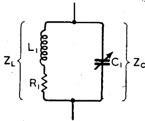
Fig. 9. Parallel-tuned circuits.
