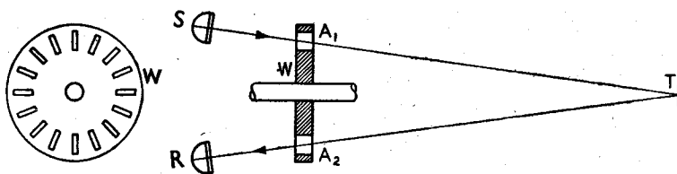
Fig. 3. Adaptation of Fizeau's classical experiment to determine the speed of light. If the speed is known, the distance A_1TA_2 can be measured by the same technique.
