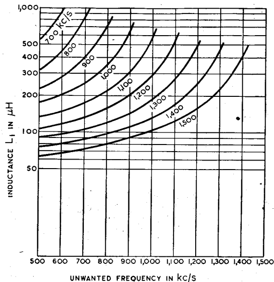
Fig. 6. Performance of shunt wavetraps. Each line indicates inductance necessary to reject frequency indicated on abscissae and boost frequency marked on curve. Aerial capacity 200 \mu\mu F .
