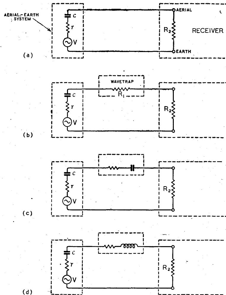
Fig. 2. Equivalent electrical circuits of a receiver and aerial-earth system (a) without a wavetrapp; (b) with a wavetrapp at its resonant frequency; (c) at frequencies higher than the rejection frequency; (d) at frequencies lower than the rejection frequency.
