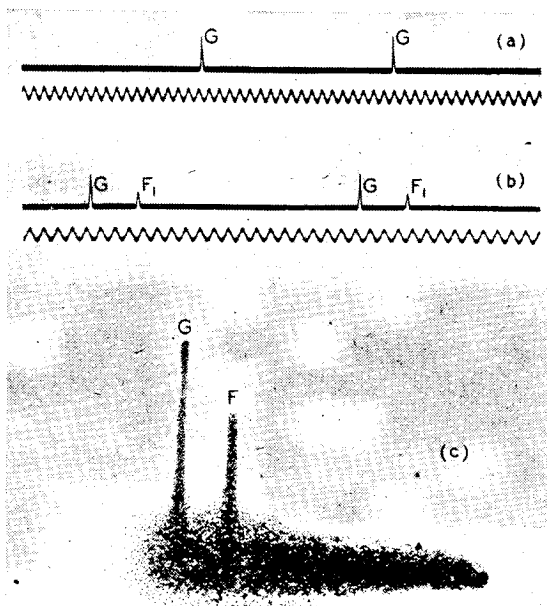
Fig. 8. (a) Record showing ground pulses only, and timing oscillation of frequency 1110 c/s. (b) Record showing ground pulses and echo received from F region about 3 milliseconds later. (c) Actual photograph of the ground wave and echo pattern as observed on the cathode-ray oscillograph screen. These records are reproduced from a paper by E. V. Appleton and G. Builder published in Proc. Phys. Soc. , 1932, Vol. 44. p. 82.
